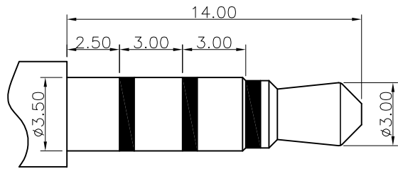
Ø3.50mm 4 POLE PLUG
